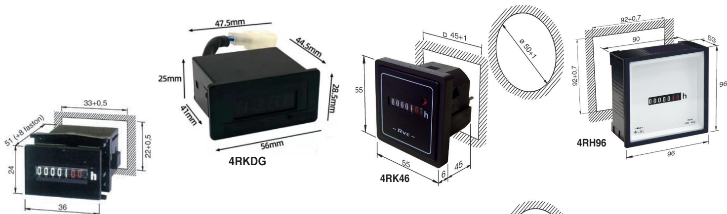
4RK30 Fast-on 6,3x0,8 mm con terminale a vite Fast-on 6,3x0,8 mm with screws terminal
